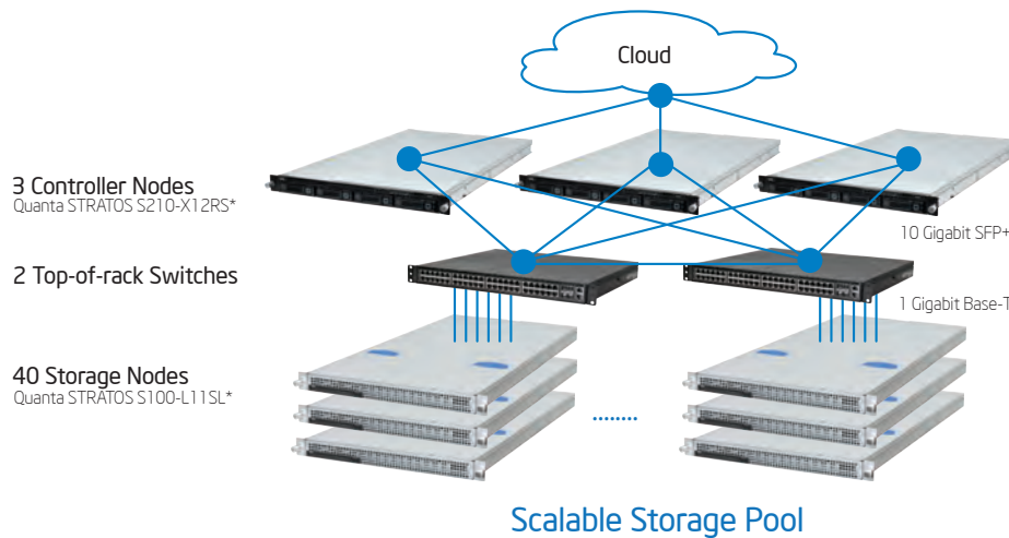
Figure 1. Sakura Internet large object store configuration.
